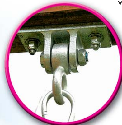
Two 3-position 4x6 Swing Beams with Commercial Swing Hangers
